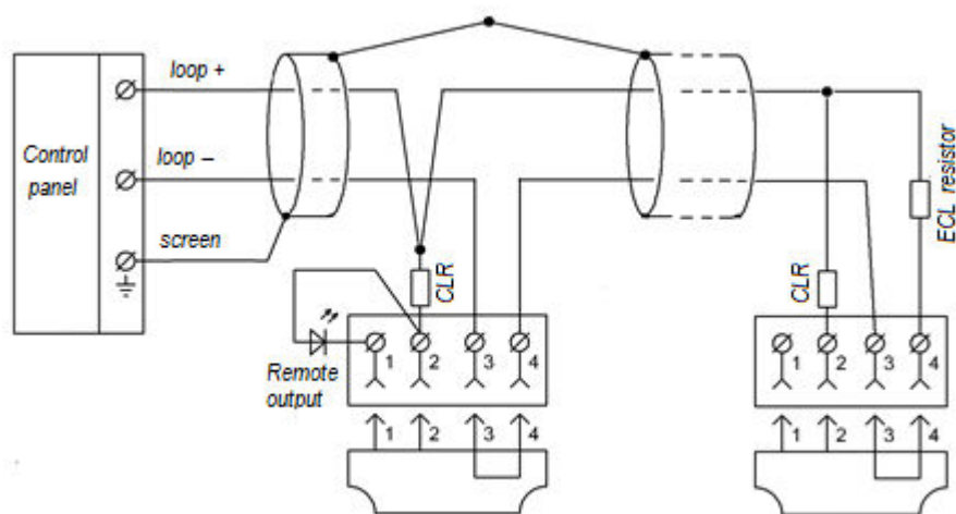
WIRING DIAGRAM FOR SPD-3.1M DETECTORS TO DC CONTROL PANEL
