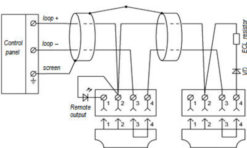
WIRING DIAGRAM FOR SPD-3.1M DETECTORS TO AC CONTROL PANEL
